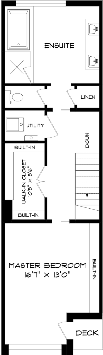
THIRD FLOOR 638 SQUARE FEET
